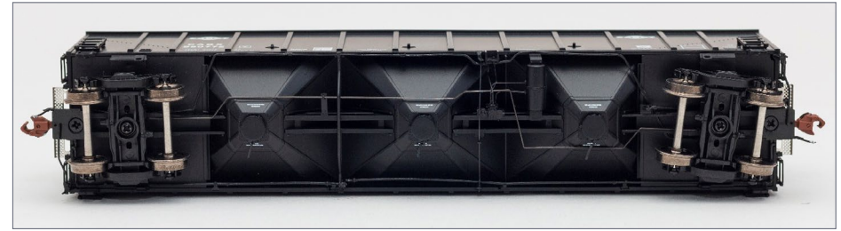
30. CABX 580772, Full underside.
