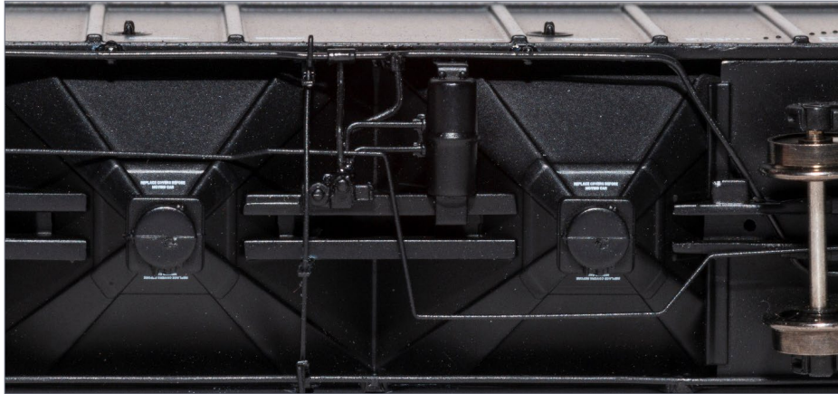
44. WITX 5875, N scale 5750 cu. ft. underbody detail.
