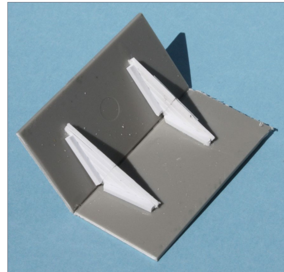
13. The roof formers shown in [12] have been glued inside the roof sheets of Pikestuff shingles. Short pieces of scale 6 x 6-inch styrene strip have been used to reinforce the joints between the formers and the roof sheets. This arrangement ensures a correct angle of the roof sheets.
