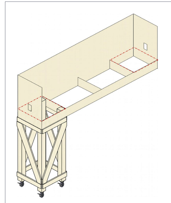
12. Be careful when mounting the supports to avoid damaging wires or turnout motors.
