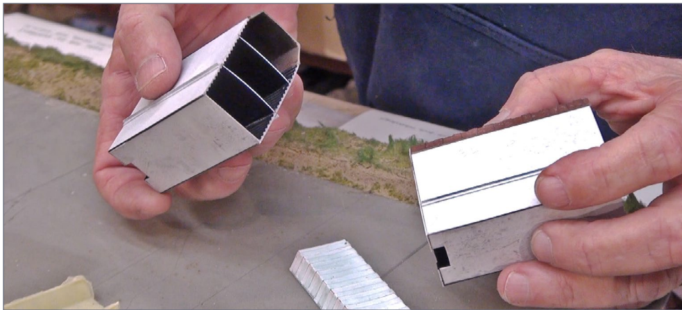
20. Mike scratchbuilt a roof section for the containers and made a rubber mold to cast 40 of them for the project. He used styrene to build simple shapes to represent the containers sides, ends, and decks in assembly-line fashion until he had 40 of them ready for paint and decals.
