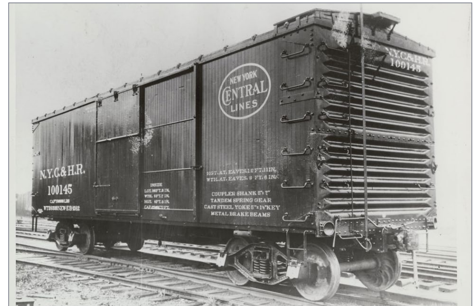
5. NYC&HR 100145, a one-off prototype box car built by the NYC's East Buffalo Shops in November, 1912.
