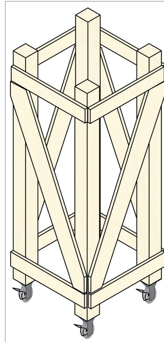
6. Module support.
