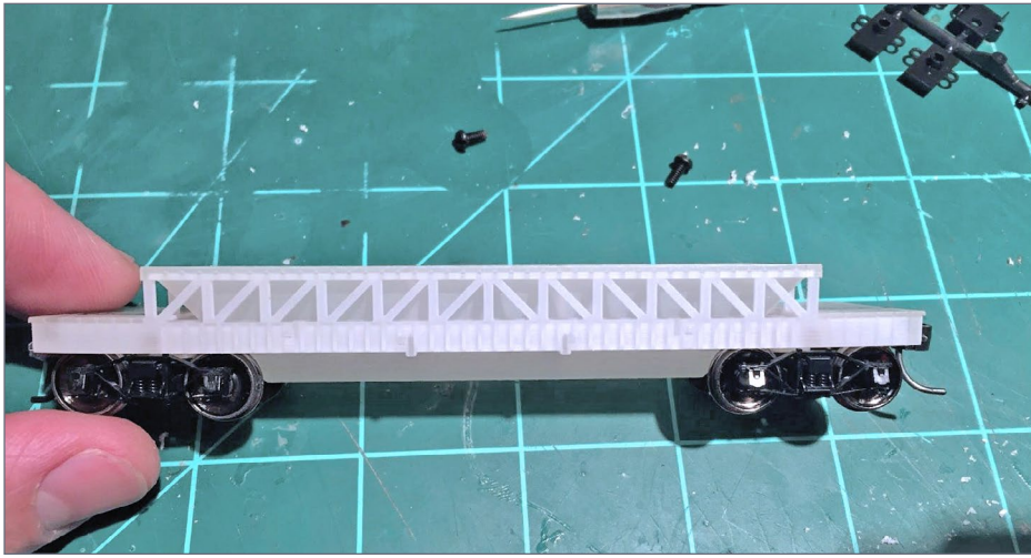
7. This side view shows the couplers and trucks attached.
