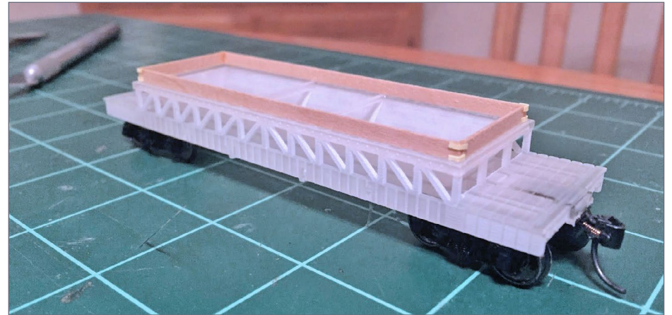
9. Here I have begun to install the details. These boards are scale 2" x 10" with pieces of paper for the corner braces.
