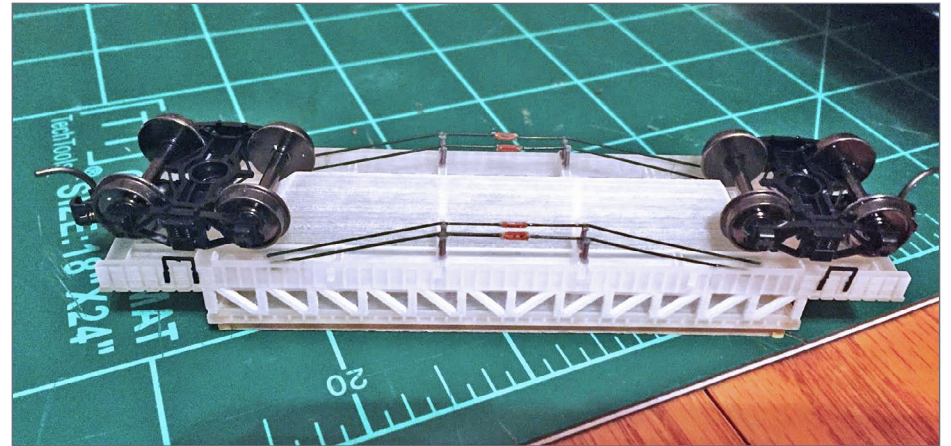
13. The floral wire was trimmed and bent, then glued to the frame to finish the truss rods.
