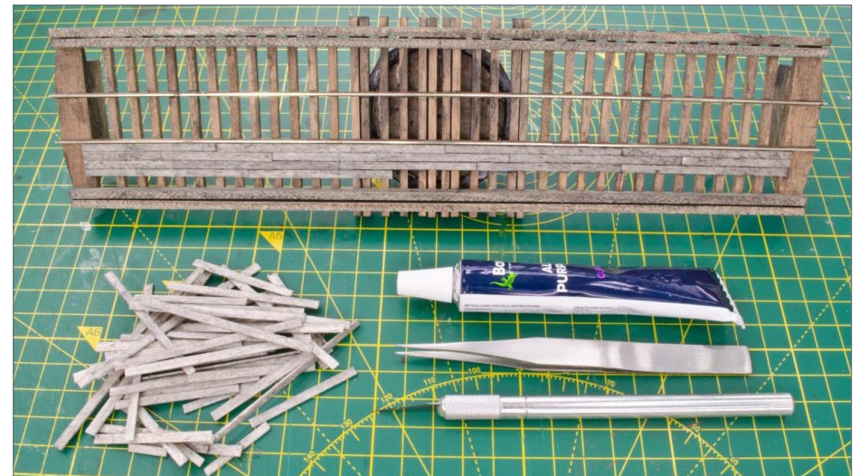
58. I made deck planking from 1/32" sheet material, cut into 1/8"-wide random lengths, which were stained with India ink and alcohol.
