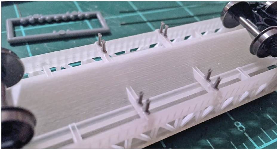
11. Tichy 10" queen posts being installed. The plans really helped position them correctly.
