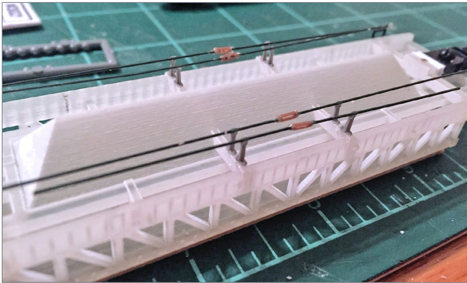
12. The turnbuckles are from Tichy as well. The ends were drilled out to accept pieces of leftover floral wire from some resin kits. They were then glued in place.
