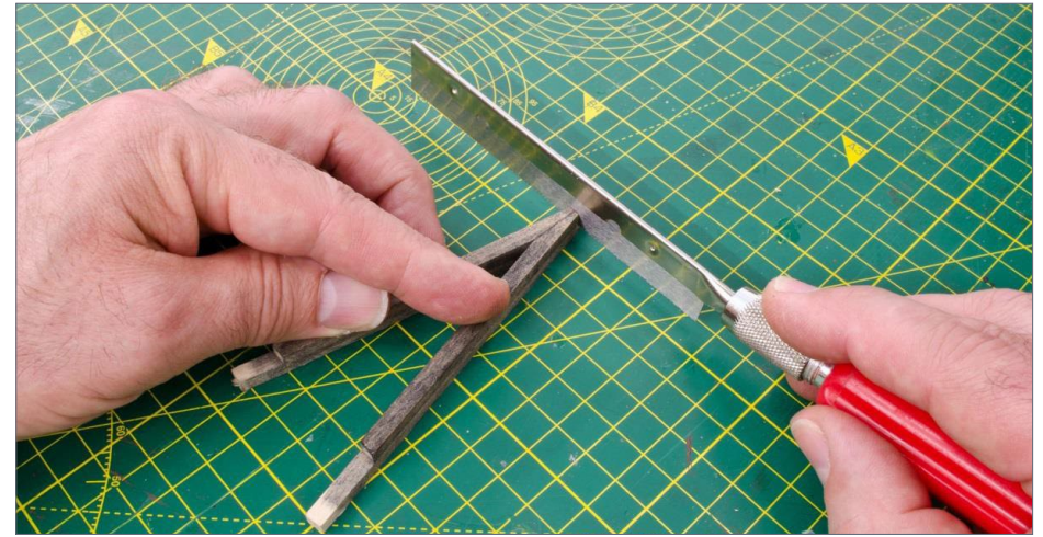
57. Using one assembly as a template for the second is a good way to keep sets square. This technique works well whenever you have identical sets, and minimizes differences.
