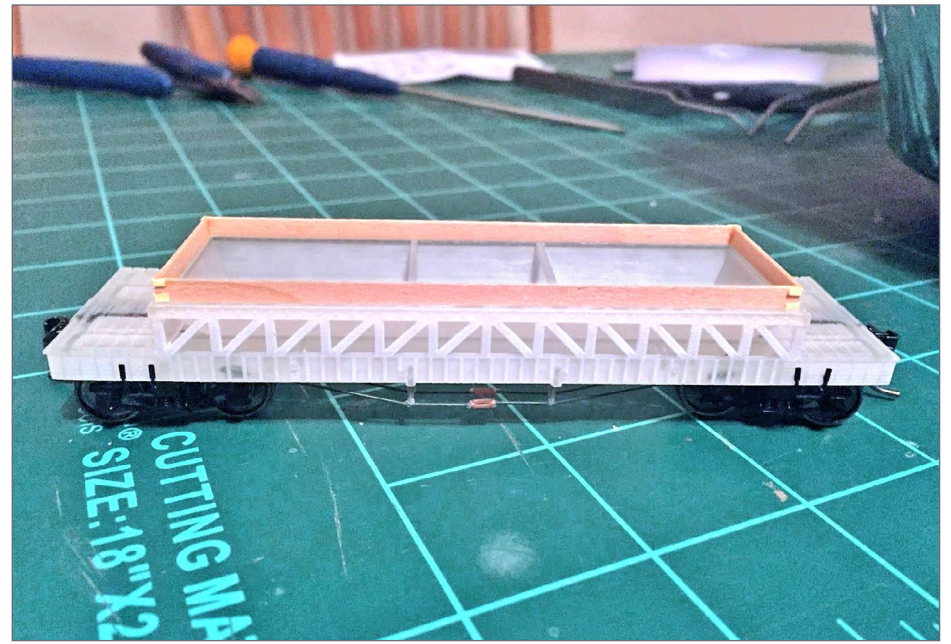
14. The finished truss rods.
