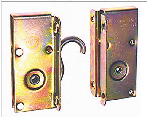
3. Norse Type 3 latch and receiver.
