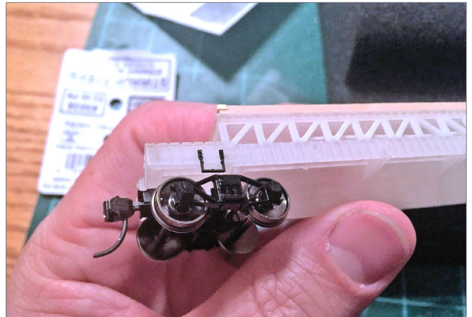
10. Tichy stirrup steps are added.
