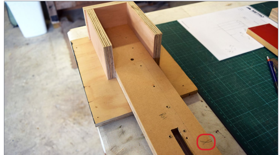
4. A simple plywood jig will align module end plates with the module end-plate in position and the “story board” on top indicating where to drill/cut. Note the facing mark (looks like a bow) indicating the top edge.
