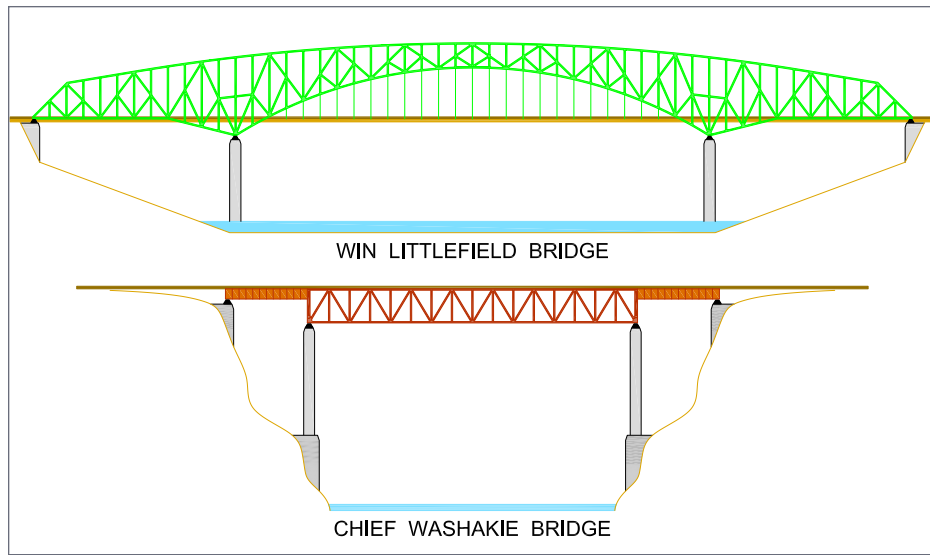
6. Scenic bridges on the SNSR.
