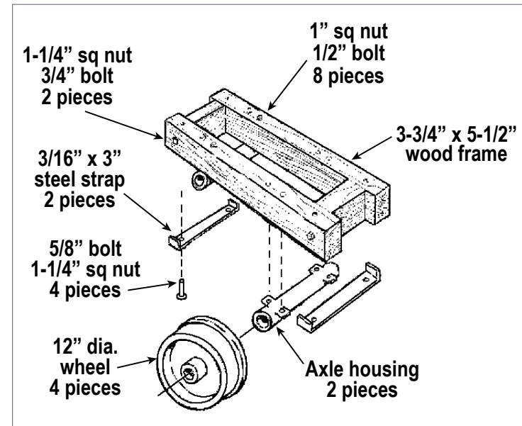
4. This perspective shows the major parts.
