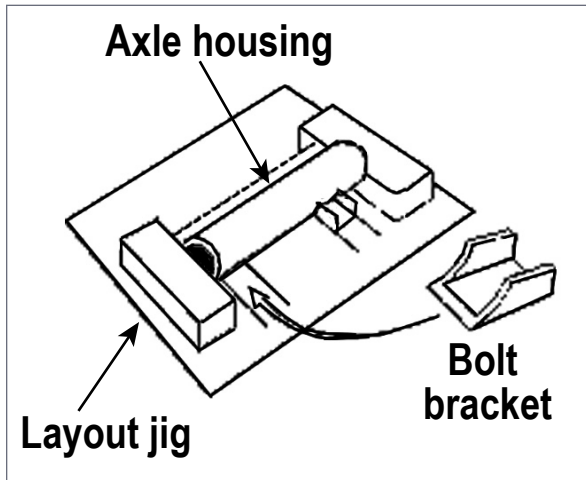
7. Jig used to add the bolting brackets to the axle housing.
