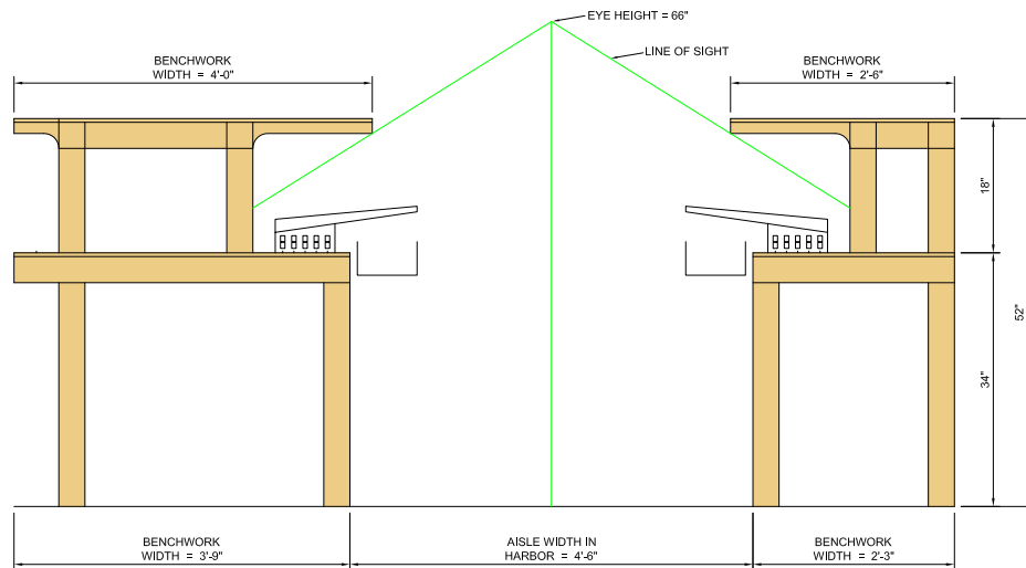
4. Typical section through the upper and lower decks.
