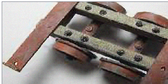
9. Note the grease boss in the middle of the axle housing.
