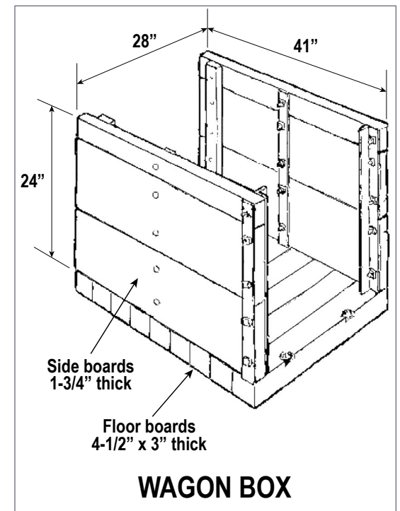
15. Wagon box details.
