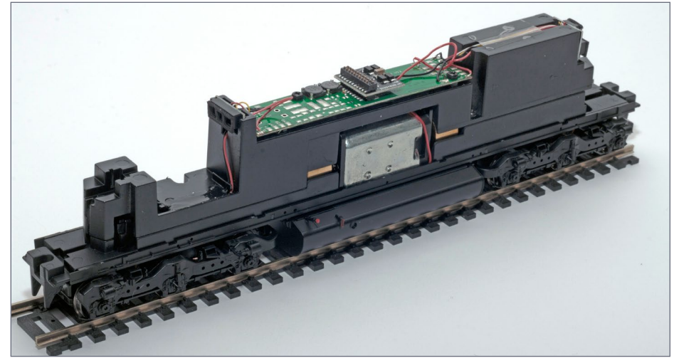
5. Operator SD40-2 chassis and motherboard with shell removed.
