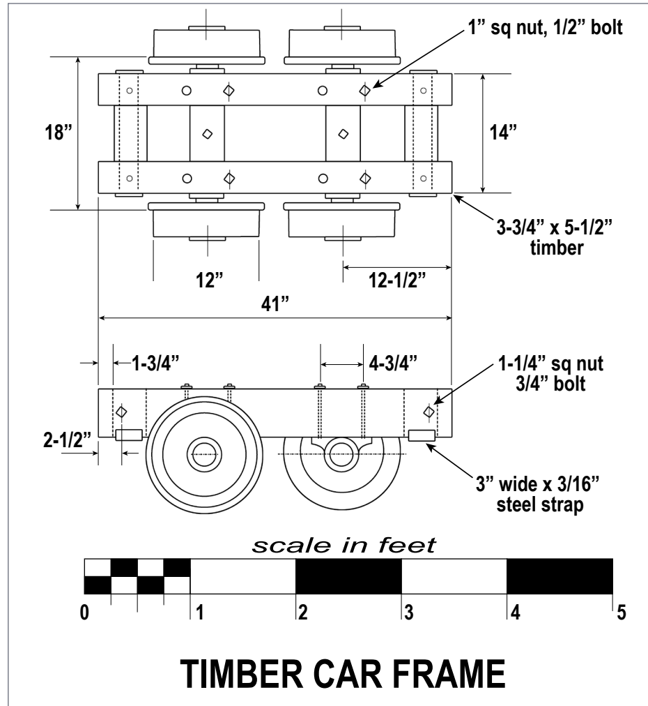
5. Plan drawing of the timber car.
