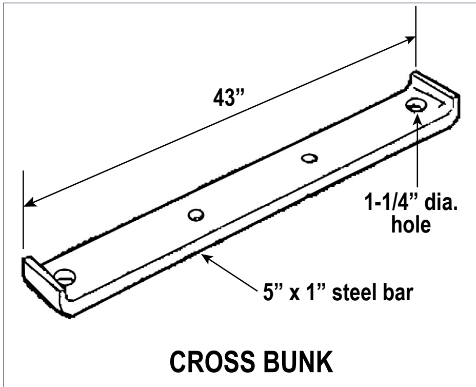
12. Steel bar cross bunk dimensions.
