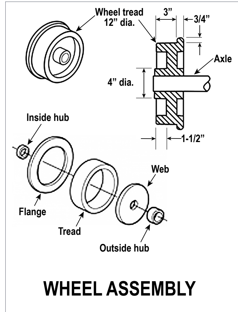
13. Wheel assembly details.
