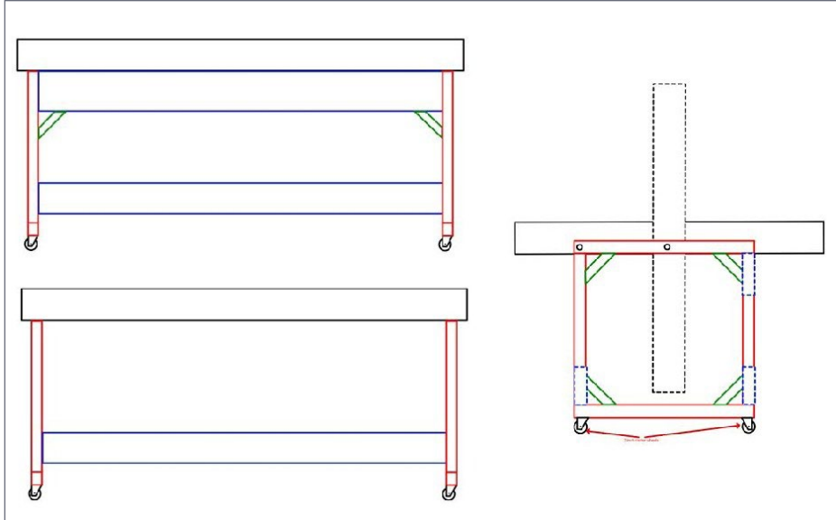
5. Drawing of the layout benchwork with the built-in tilting mechanism.
