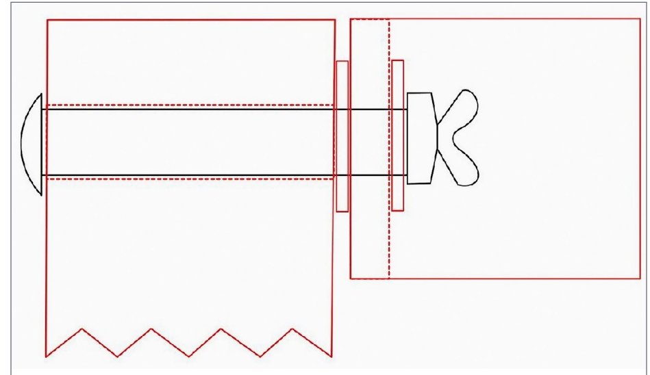
6. Bolt inserted through center hole, with a wingnut on the end. Insert a washer between the table and frame, and between frame and nut.
