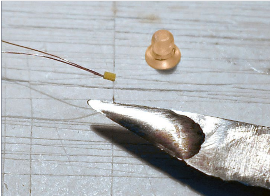
15. Quickly glue the LED into the globe with CA.
