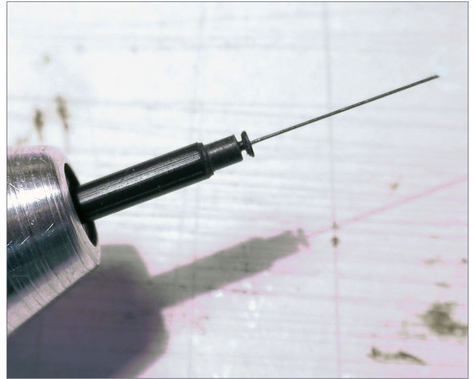
27. Glue a wire into the hole of the lamp base.
