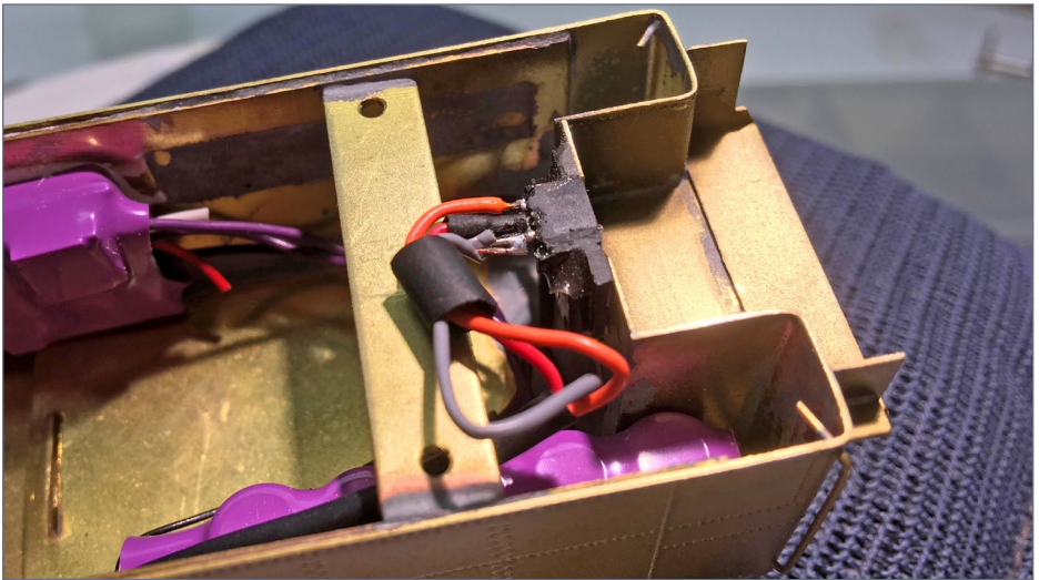
4. Three-pin female connector wired to tender side. Bruce Petrarca photo
