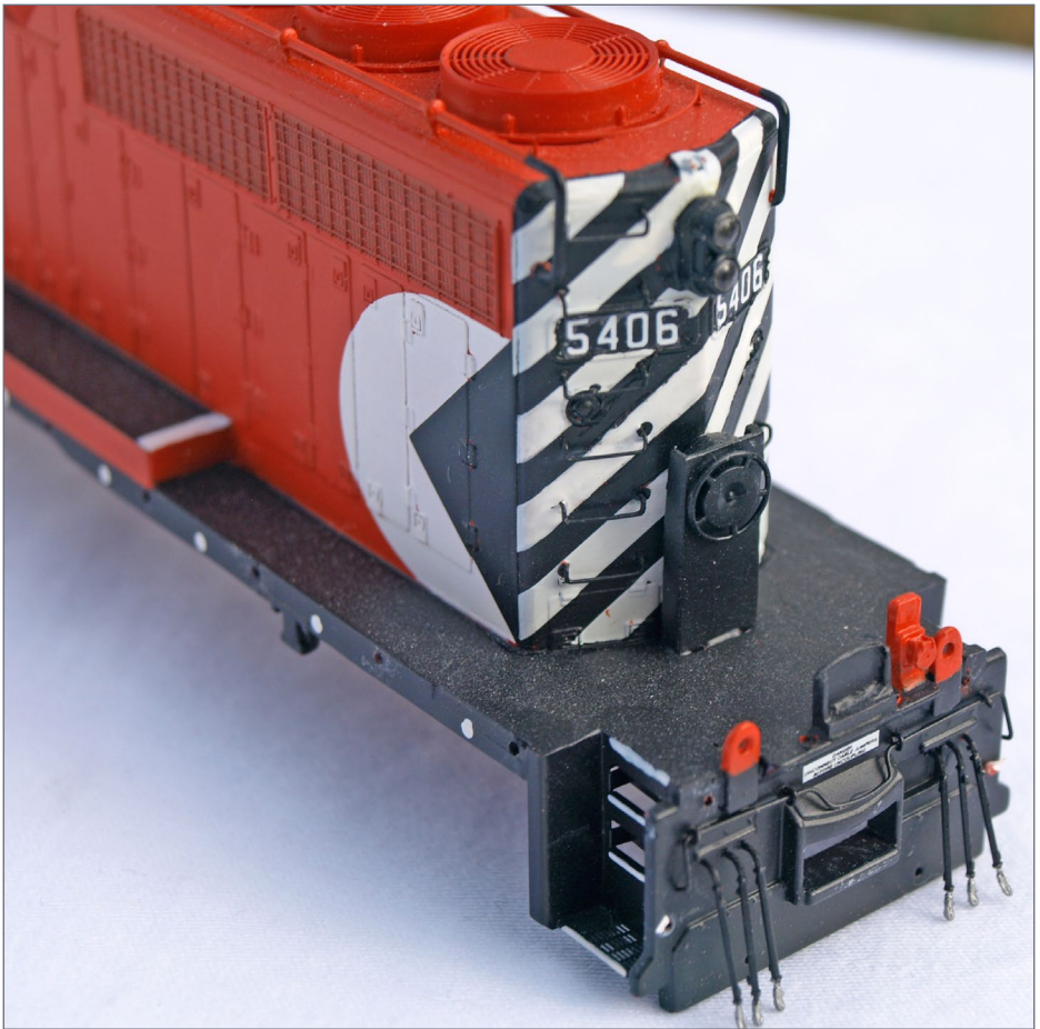
12. Rear pilot details and brake stand.
