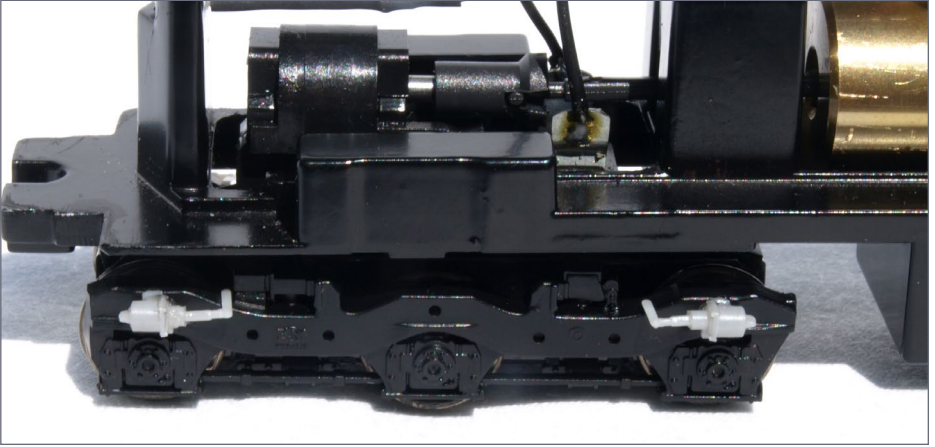
7. Brake cylinders on trucks.
