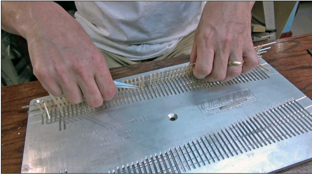
7. After the glue cures for five minutes, Jeff gently pulls the turnout out of the Jig in one piece.
