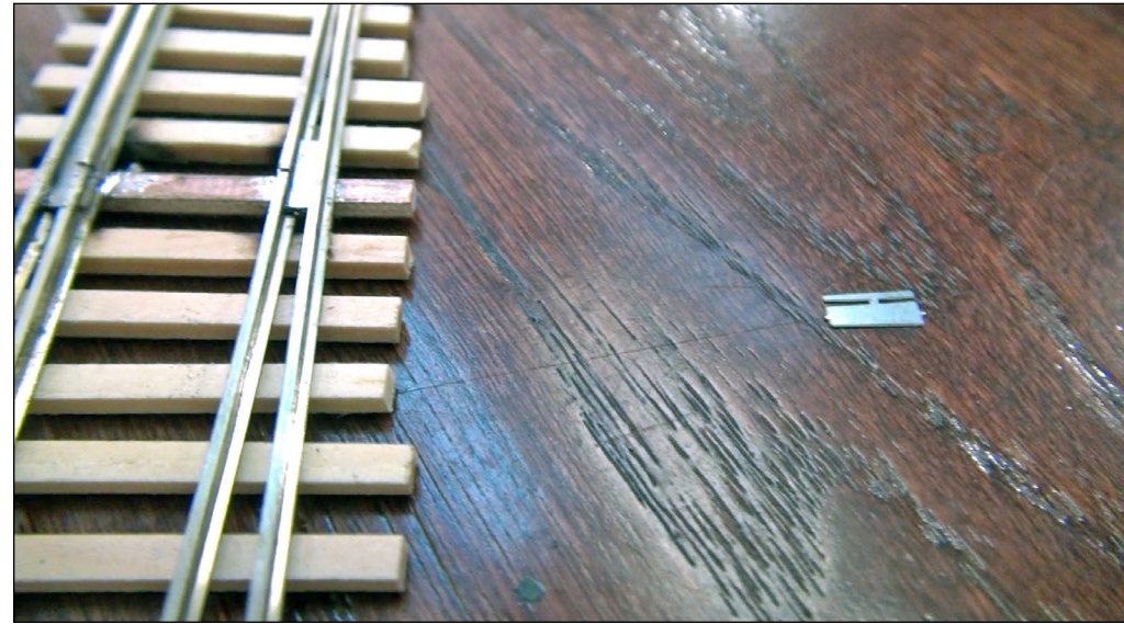
8. Here is the turnout with the hinge installed attached to the points and the adjoining rail. Alongside the turnout is the hinge as flat etched stock before it is bent and soldered to the rail. This flex point conducts the power to the switch point rails.
