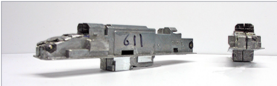
22. Reduce width of frame fuel tank area by filing it down. Original width illustrated on right.
