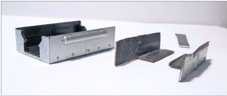
27. Original (left) and modified (right) fuel tank sections.
