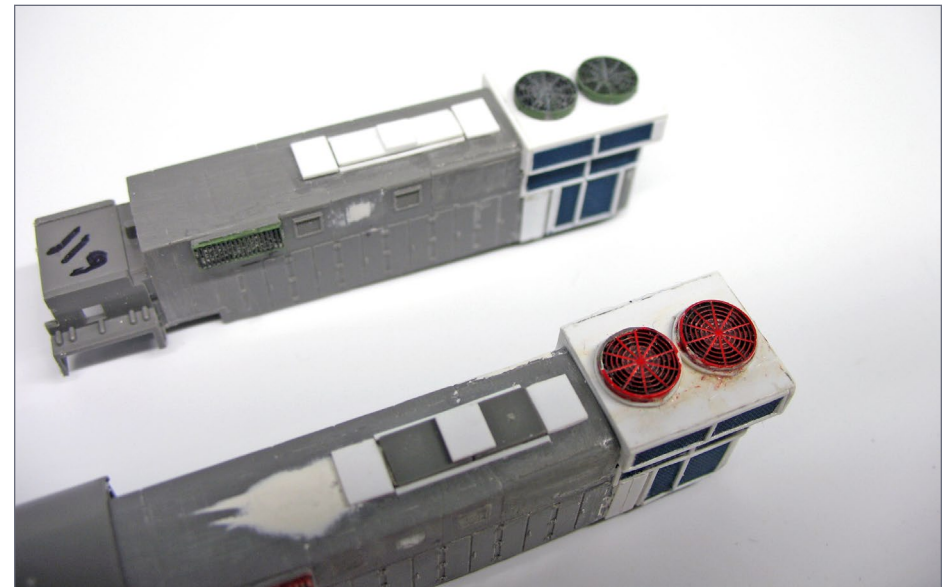
9. Form roof hatch detail from removed RS-11 details and strip styrene. Top unit has roof hatch detail built entirely from styrene. Bottom uses a combination of salvaged RS-11 hatch detail and styrene.
