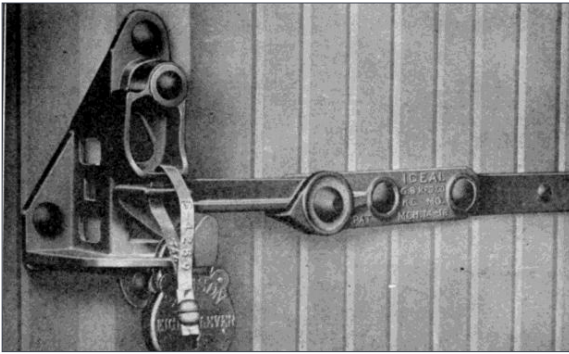
61. Automatic freight car door lock by Gustin-Bacon Co. circa 1910.
