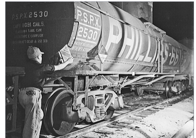
27. A workman in this John Vachon photo is inserting a “DANGEROUS” placard in the holder on a loaded Phillips Petroleum tank car. The placard holder to his right still has the empty placard from the previous trip; sometimes the black-white division in the diamond was placed horizontally, as here. Photo taken at the Phillips gasoline plant in Borger, Texas, November 1942. (Library of Congress, negative LCUSW3-011653)
