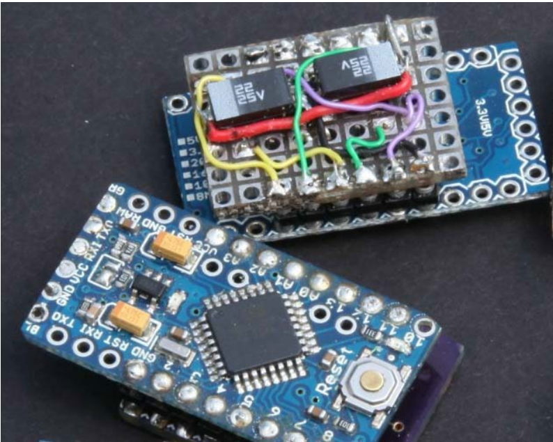
74. Hand-built driver board.
