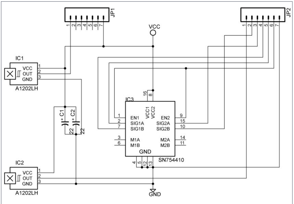
69. Dual motor driver schematic.
