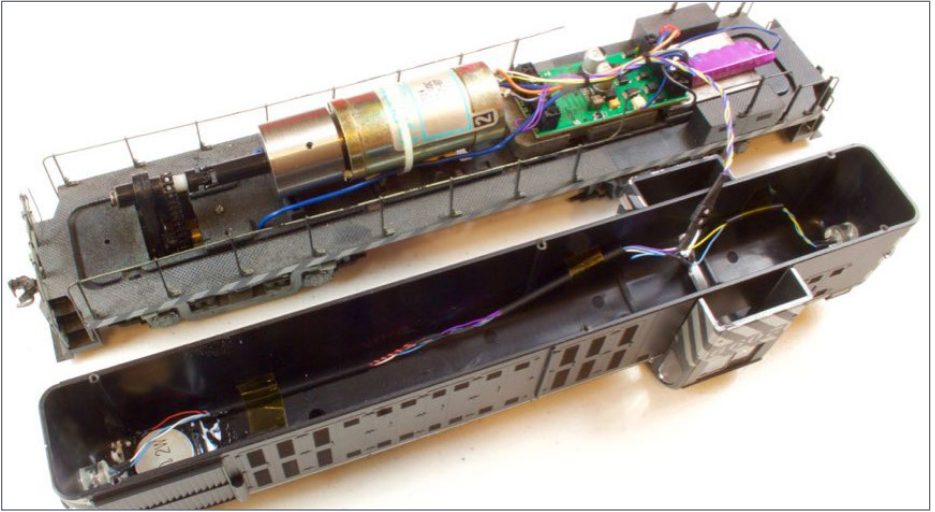
15. Overall view of completed installation.
