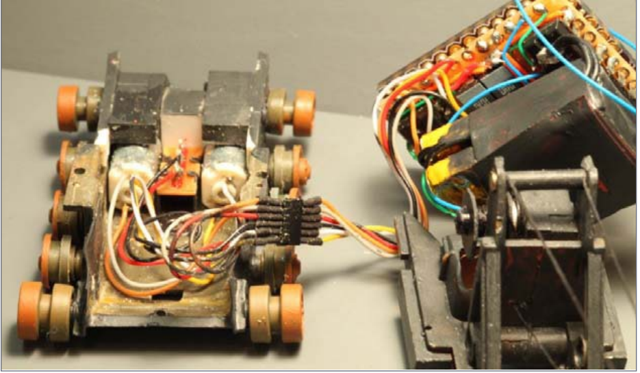
88. Crane 3 motors and wiring harness.
