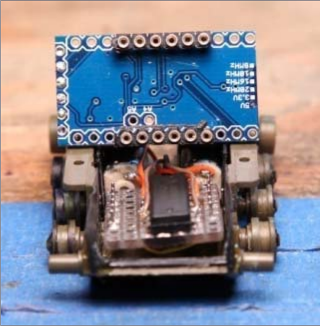
75. Hand-built driver placement in the chassis.
