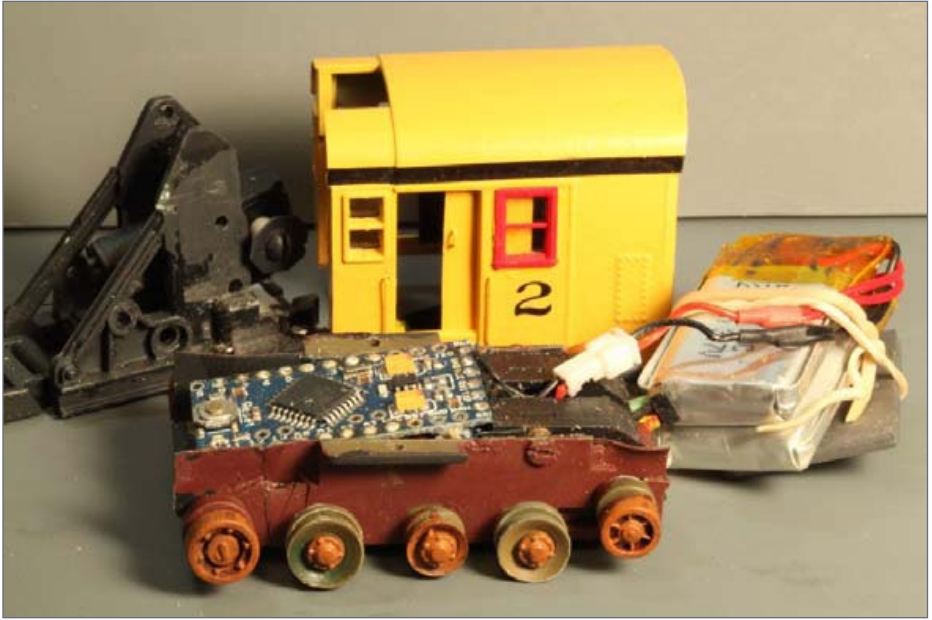
80. The cab is ready to be mounted.
