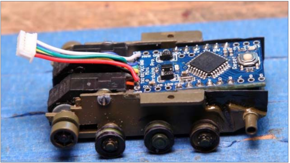
76. Progression of chassis construction.
