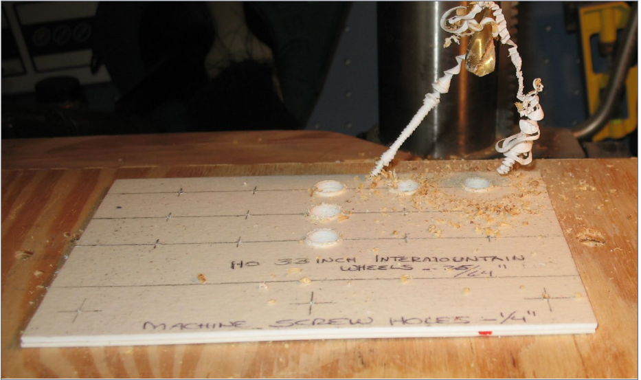
7. Drilling wheel mask holes.
