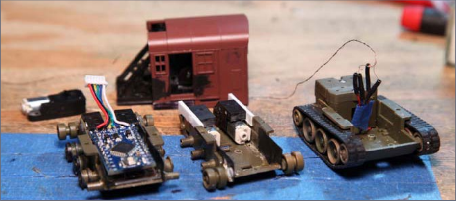
73. Progression of chassis construction.
