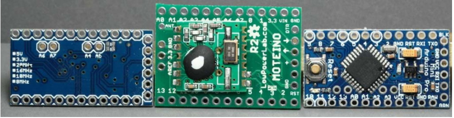
83. Arduino Pro Mini (left) vs. Moteino (right), bottom view.
