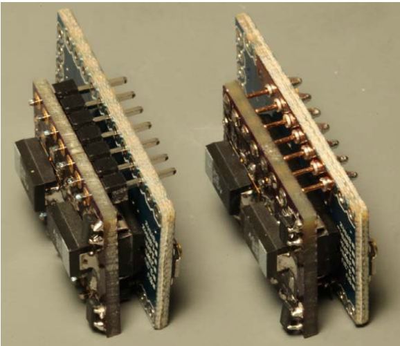
72. Motor driver attachment alternatives.
