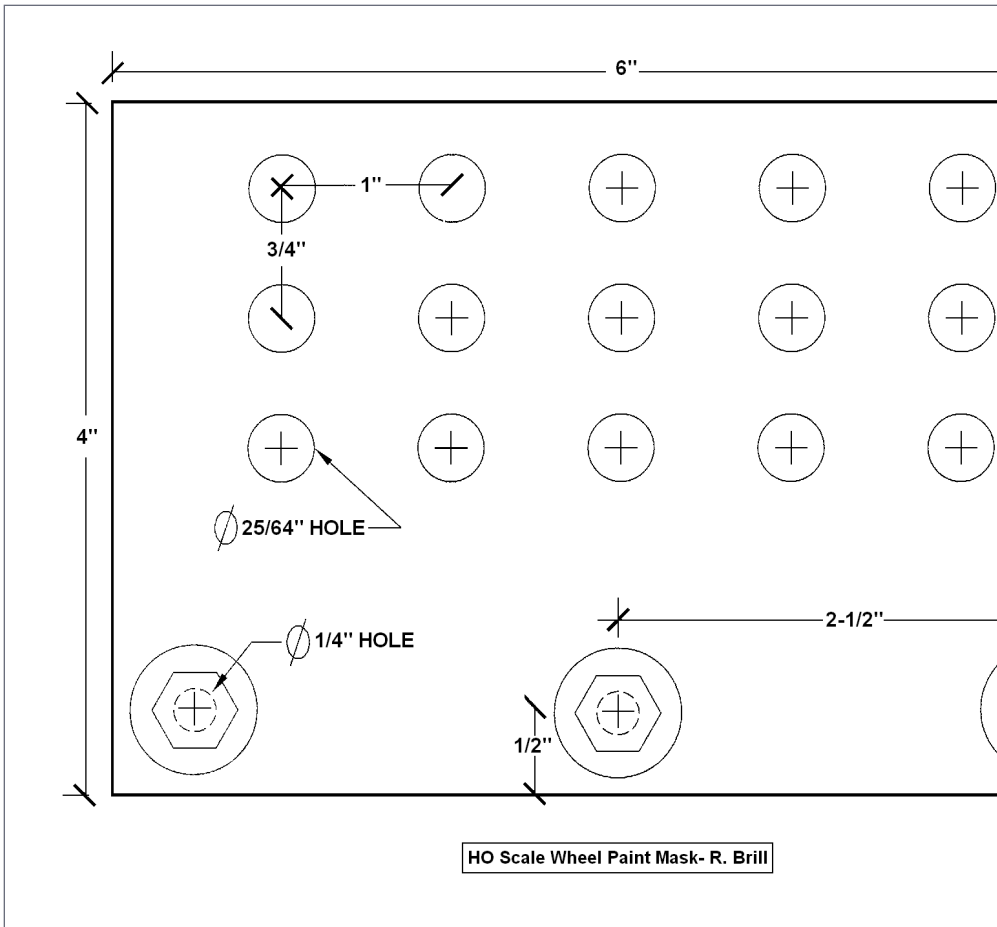
Wheel mask drawing.
