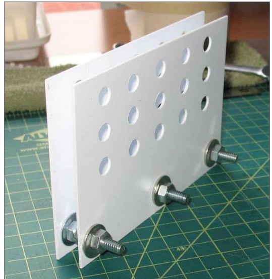
12. (Left) Assembled wheel mask side view.
