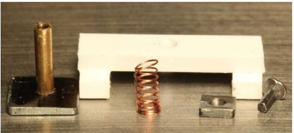
97. Putting the box together.
