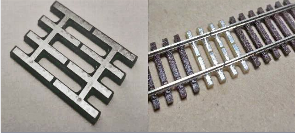
2. This Gapmaster is installed on N scale Micro Engineering Code 55 flex track. American Tie & Timber Co. photo
