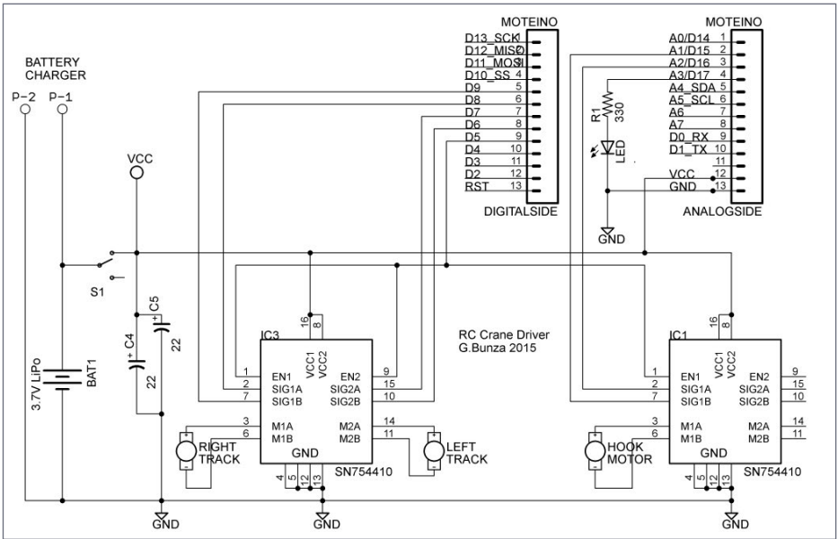
84. Crawler crane schematic.
