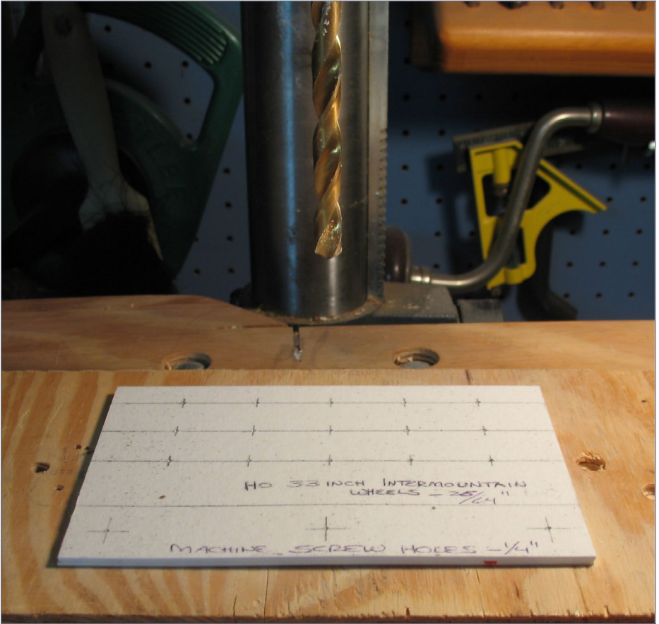
6. Marked sheet set positioned on scrap wood ready for drilling.
