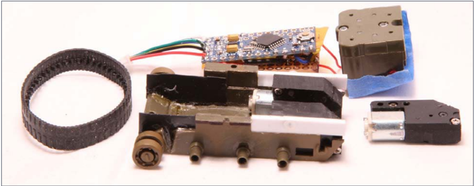
59. Chassis parts.
