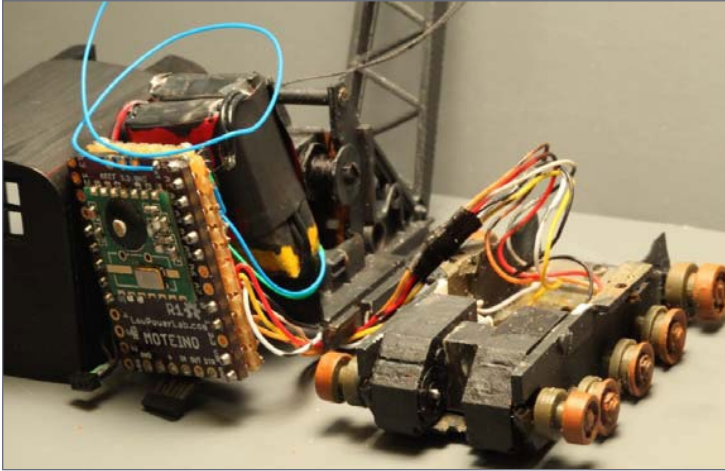
87. Crane 3 internals.
