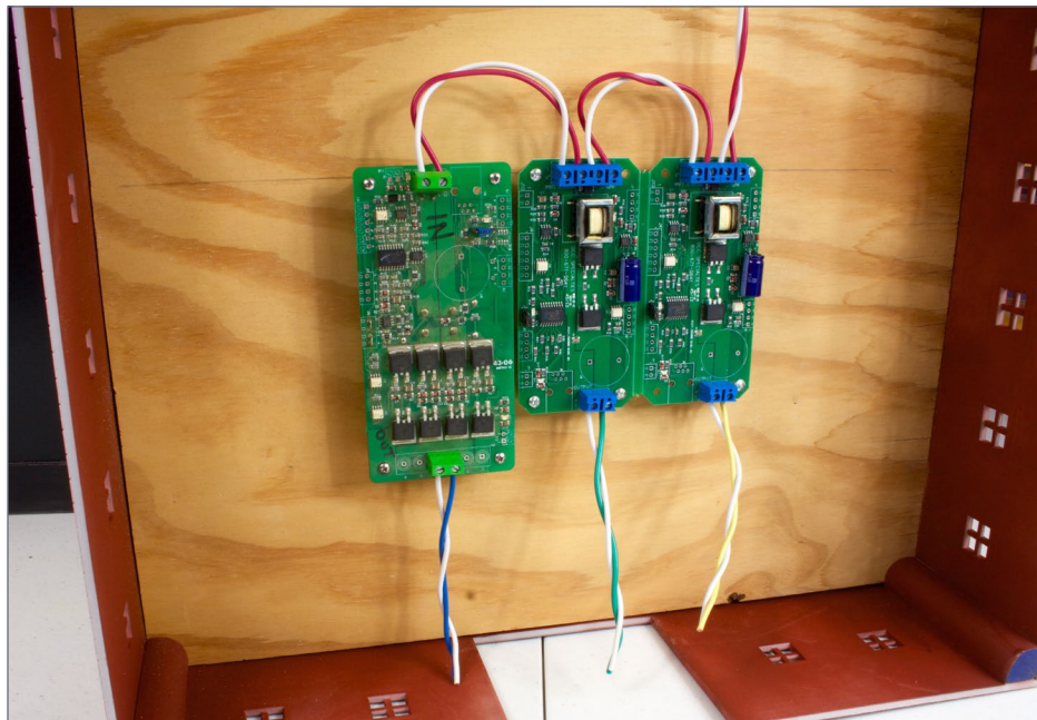
4. Electronics in a barn viewed from the bottom – wires are just for testing and do not conform to the color codes used in this column – an 8-pin connector will be added.
