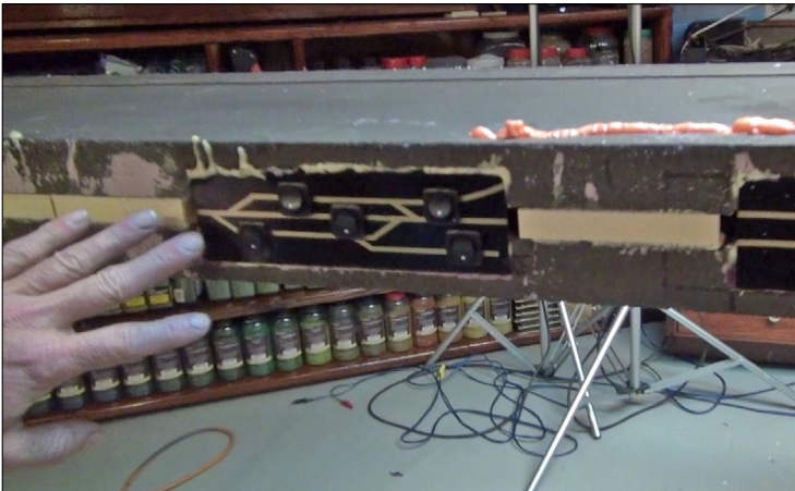
12-13. Embedding layout wiring in foam to hide the wires.
