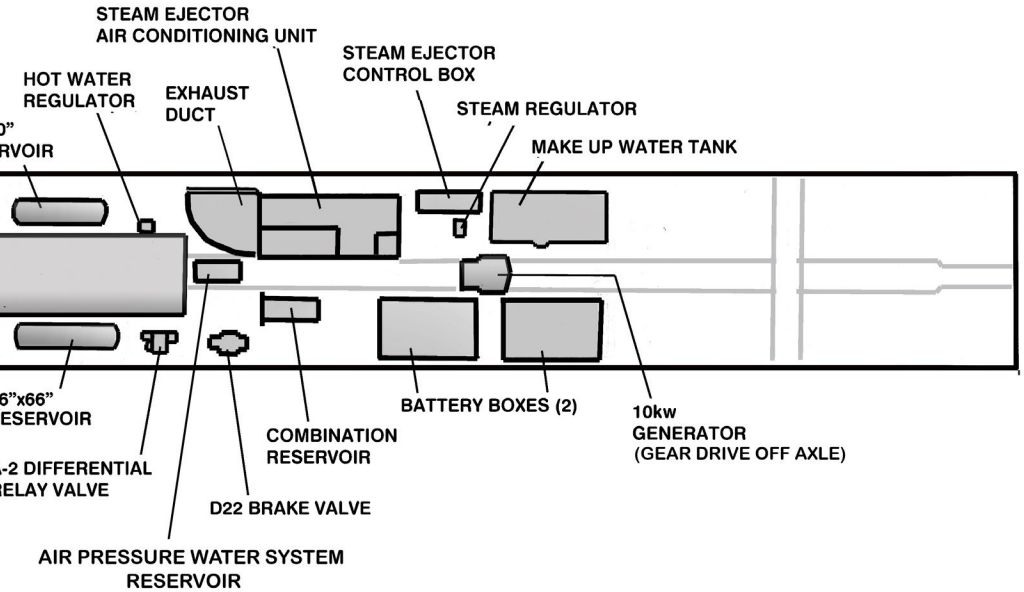
FREE SHOP-TAVERN CAR (CLASS 77-T-1) SHOWN AS EXAMPLE
