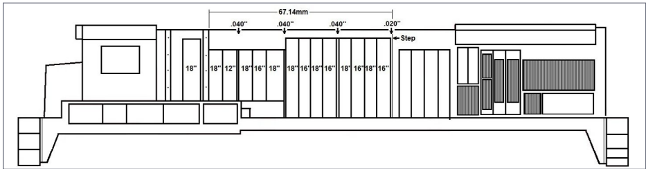
13. Last door.
