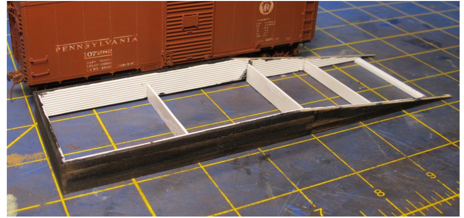
13. Testing the height of the completed frame. The top of the frame should be level with the boxcar floor. The model is a kitbashed HO scale Branchline PRR X26B.
