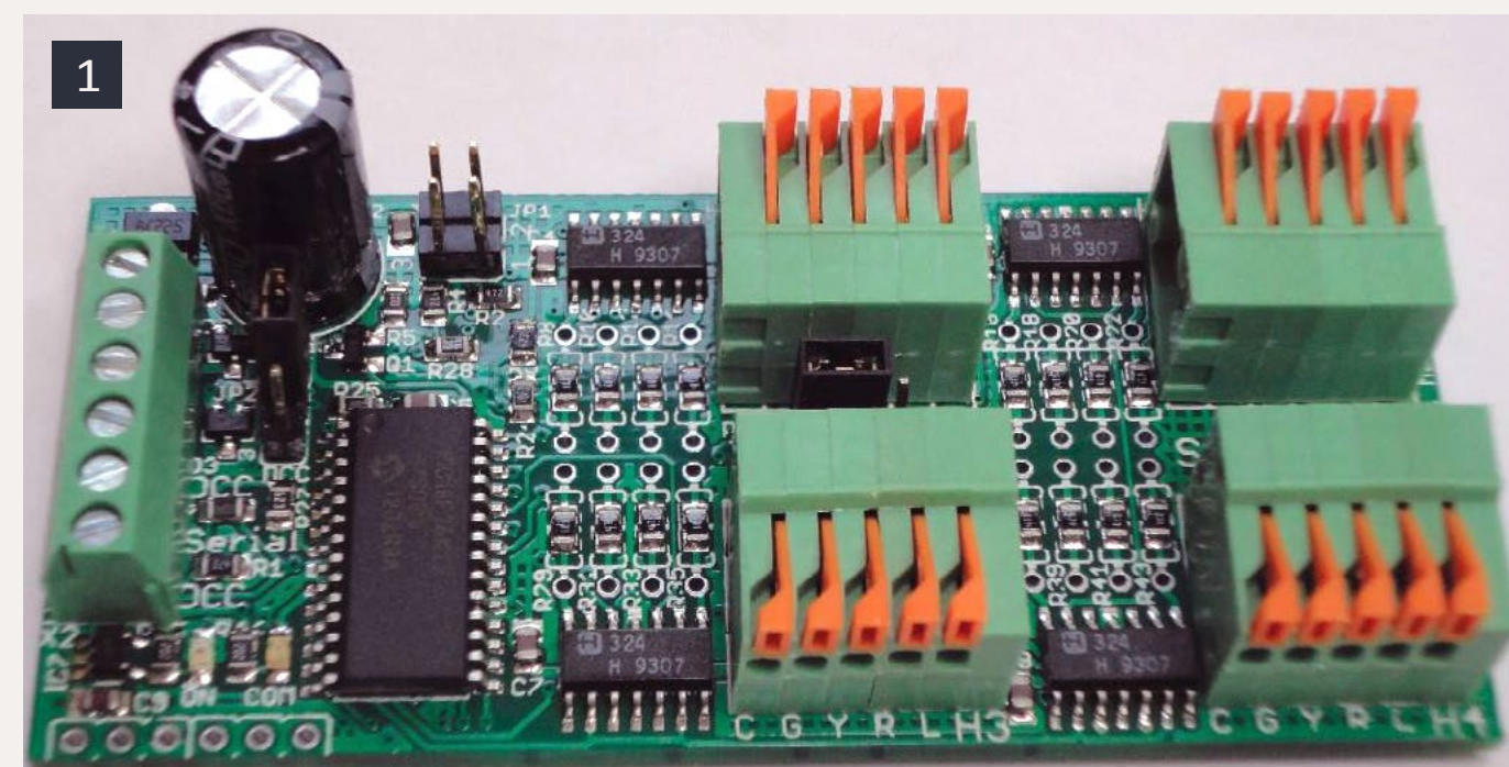
1: SignalMan C (compression connectors version).
