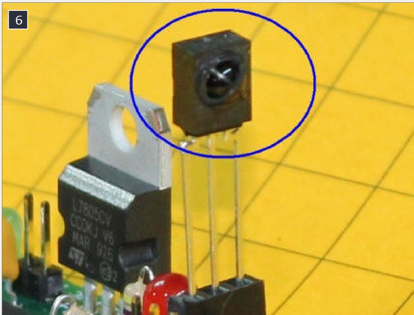
6. The small Vishay TSOP4838 chip receives the infrared codes.
