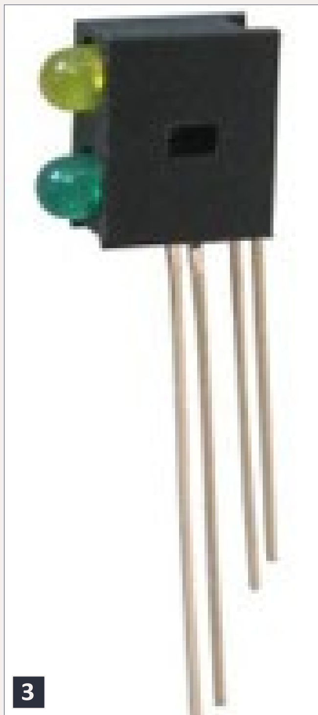
3: A bi-level LED assembly suitable for a track-side signal as is. Photo courtesy of All Electronics.
