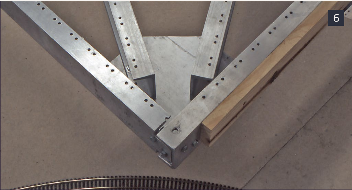
6: Looking down on mid level horizontal corner framework. Gussets are used to attach the parts together instead of attempting to bevel cut the angled pieces. This type of construction is very similar to steel framing in buildings. The outside corner framework has 1x3 wood attached. Sub-roadbed and risers are mounted to the framework using this wood piece.
