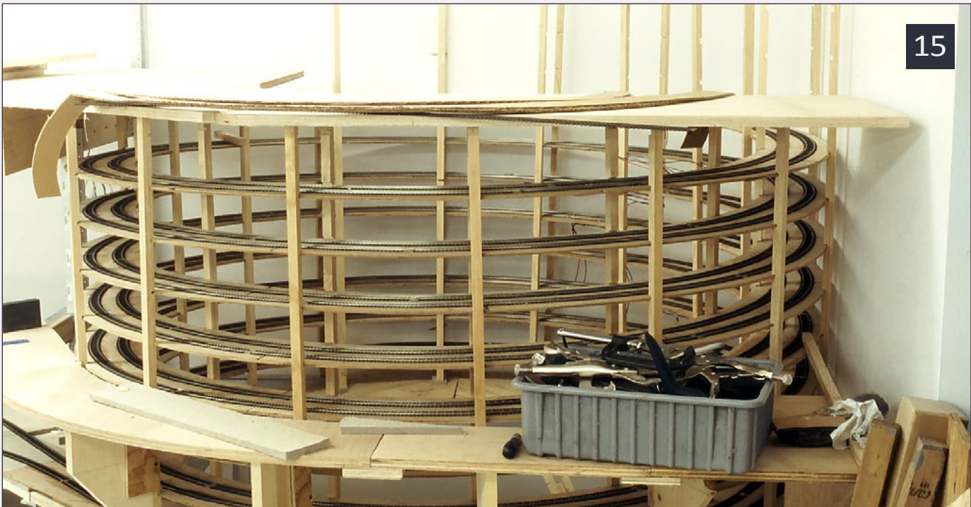
15: Some of the vertical risers of the helix have been trimmed to their final height. The mid level area with the tool bin is the Coalgood branch. Above it is the sub roadbed for Eljobean.
