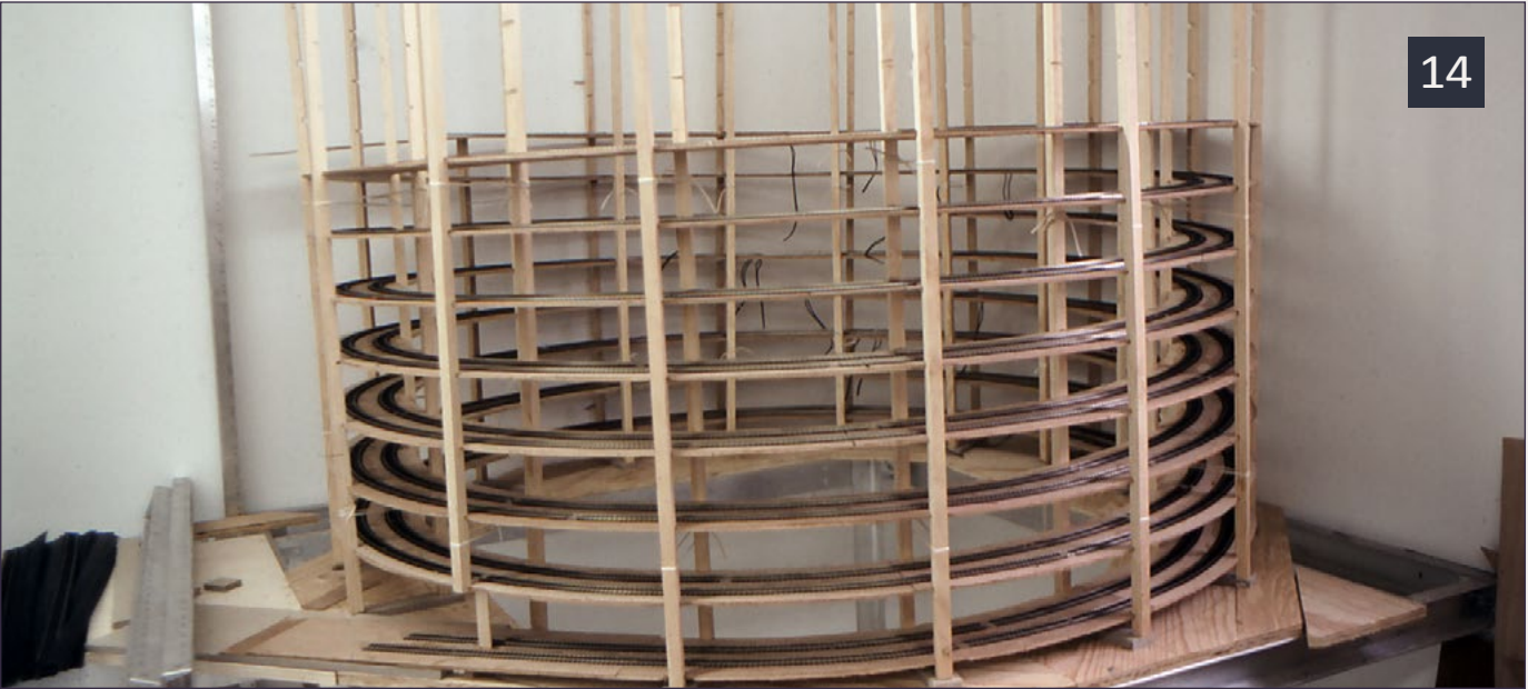
14: Helix B is under construction. The helix's roadbed is made with 1/8" door skin plywood.
