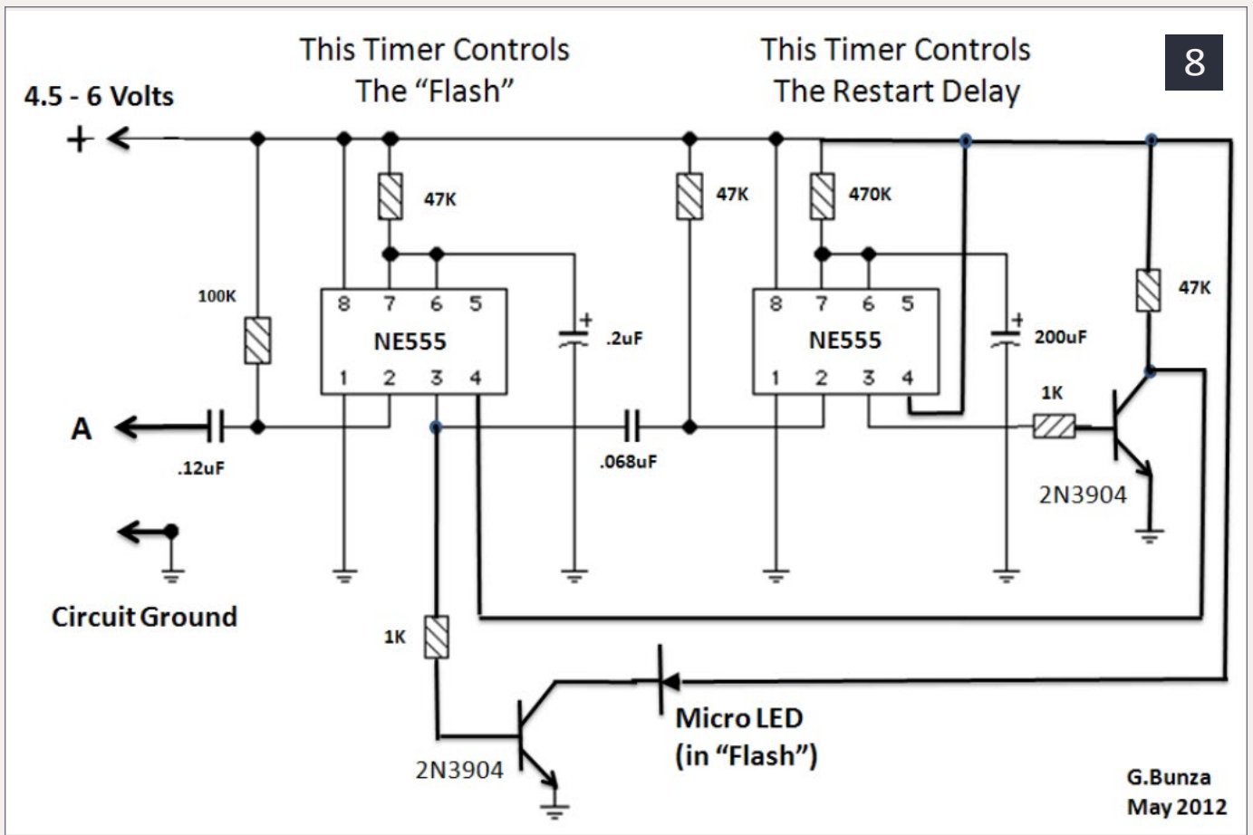
8. Flash timer and delay circuit schematic.
