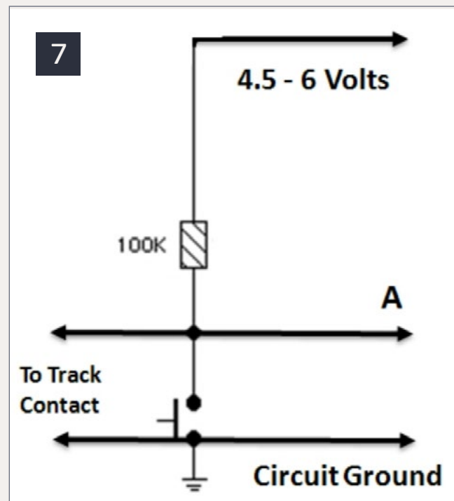
7. Track contact circuit.
