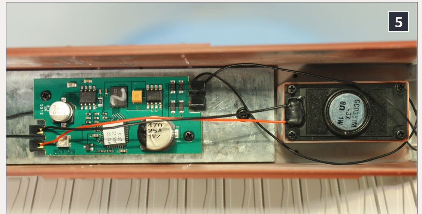
5: Volume control on installed sound board, and speaker.
