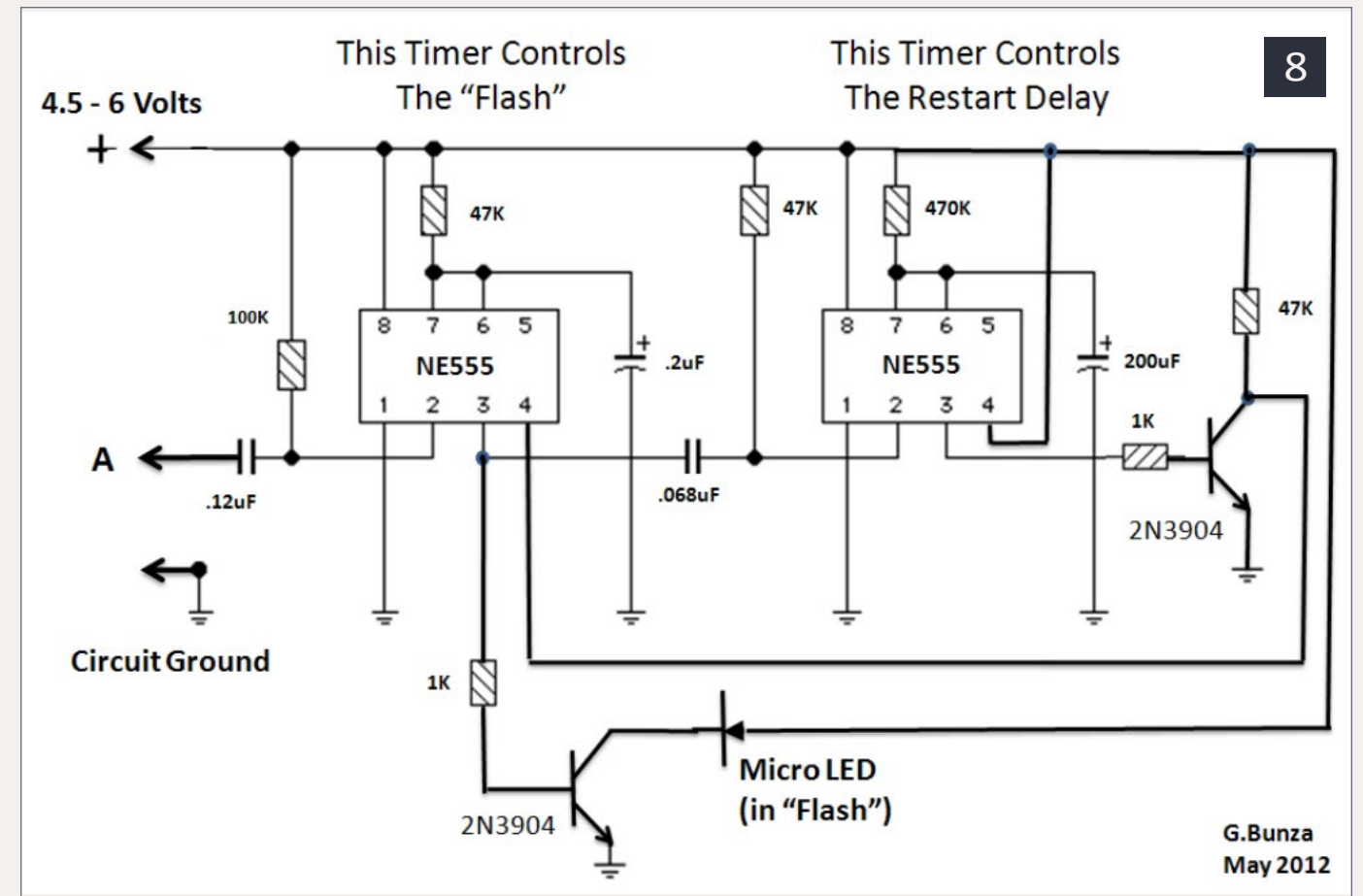
8. Flash timer and delay circuit schematic.
