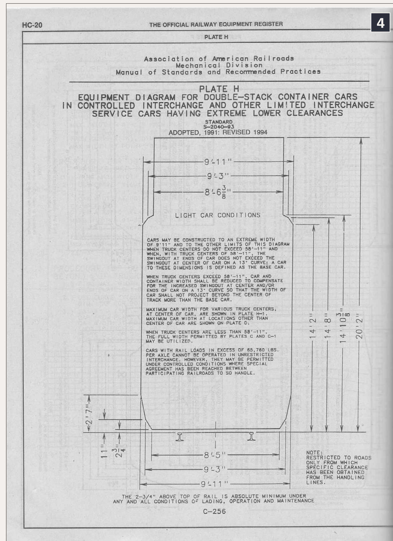
4: AAR plate H clearances for interchange, from the Official Railway Equipment Register.
