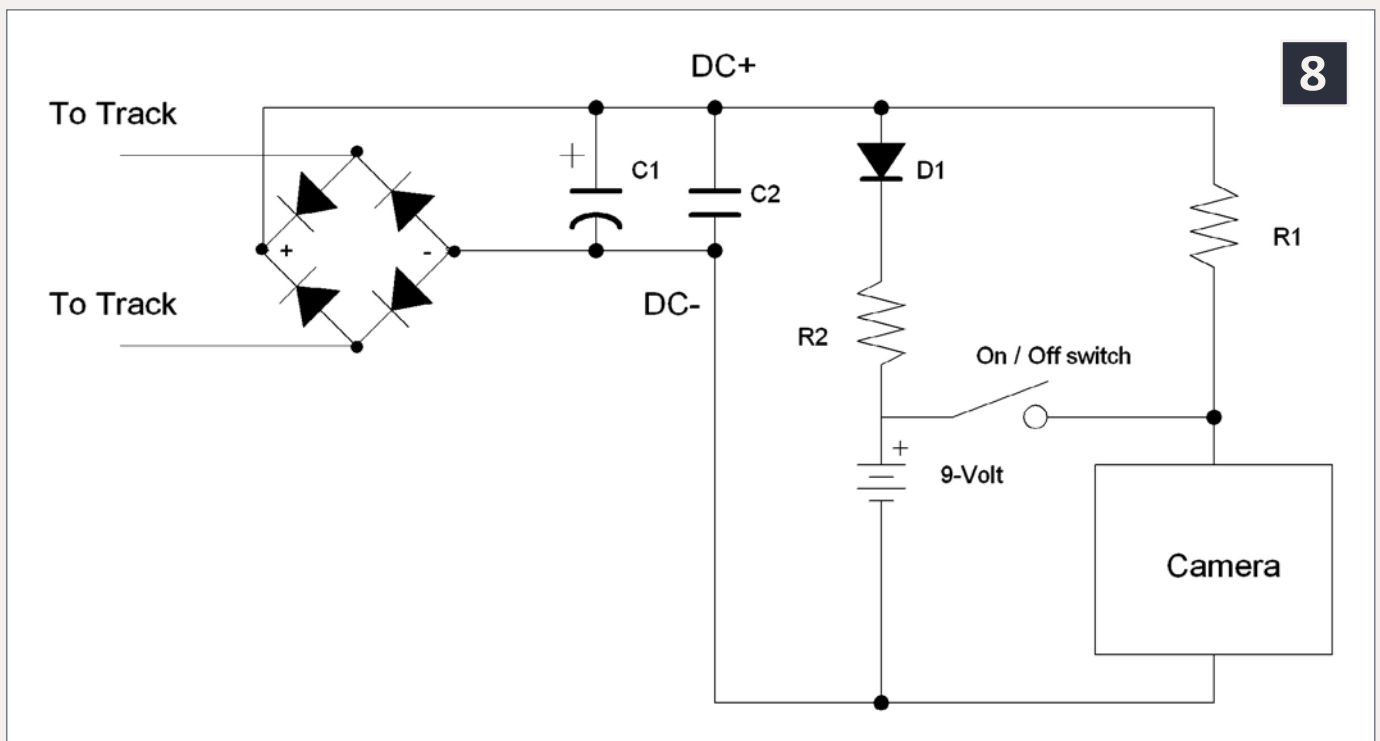
8: Complete circuit diagram.
